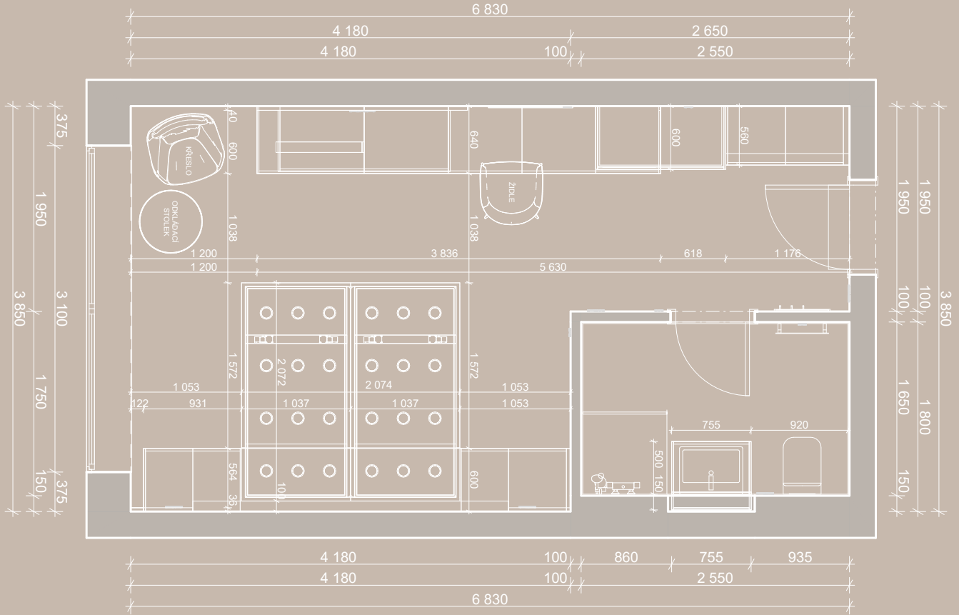
Floor plan
